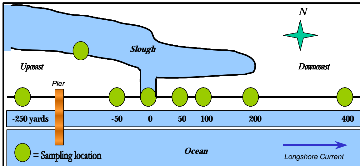
Figure 4.2. Schematic of Sampling Stations at Goleta Beach/Slough.
