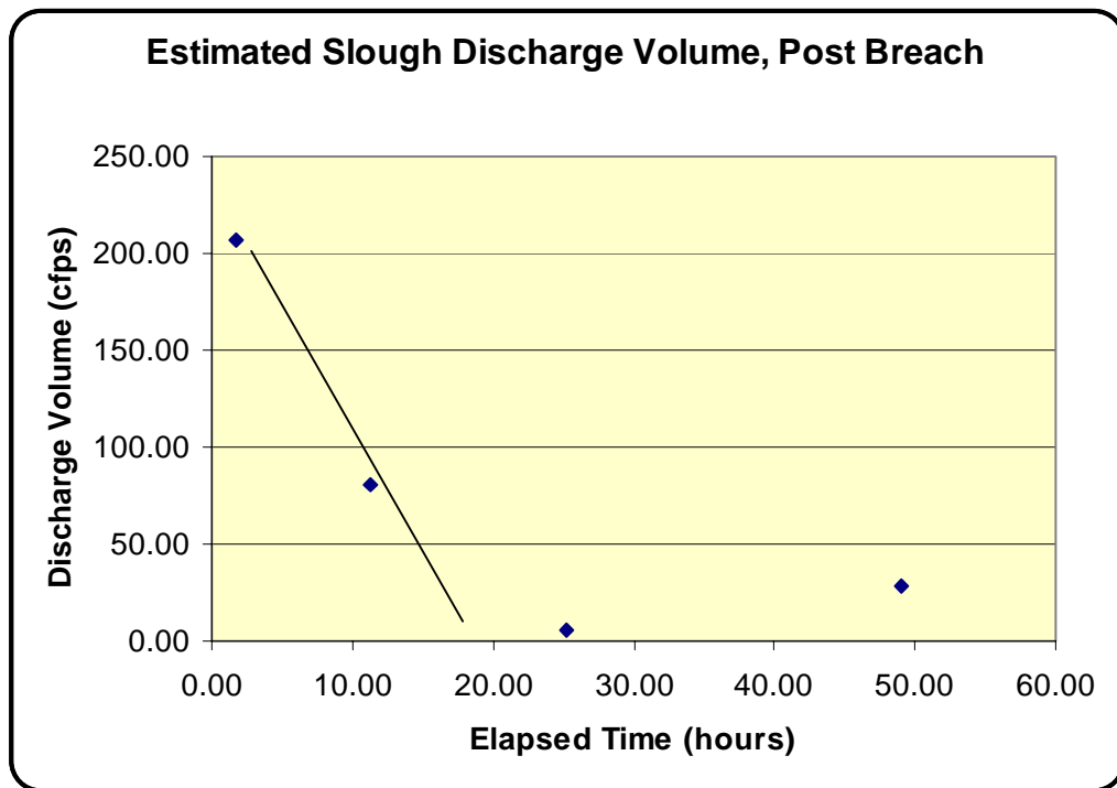
Figure 5.16. Estimated Discharge Volume Rate versus Elapsed Breach Time
