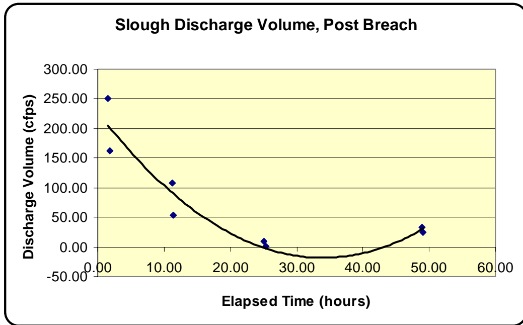
Figure 5.5. Estimated discharge volume versus elapsed time from the breach.
